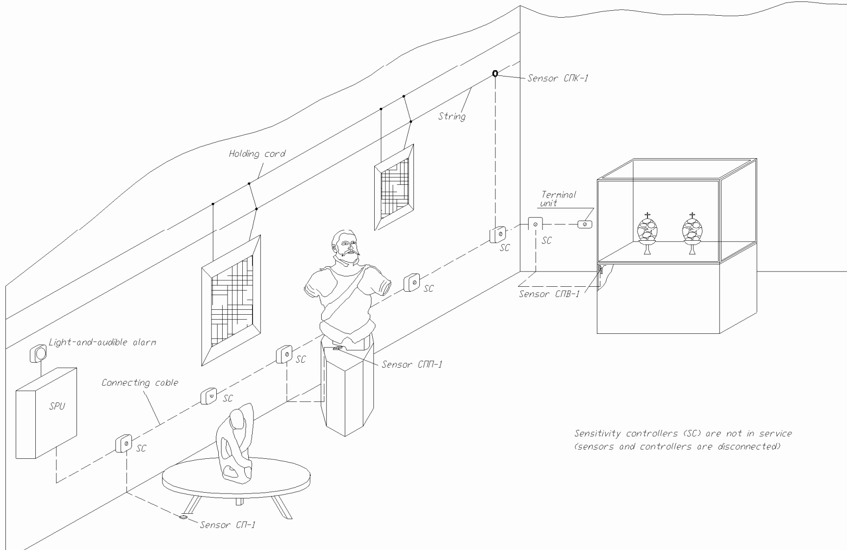
- Fig. 3 - Example of Using Burglar Alarm for Equipping Exposition Hall with Changeable Display
