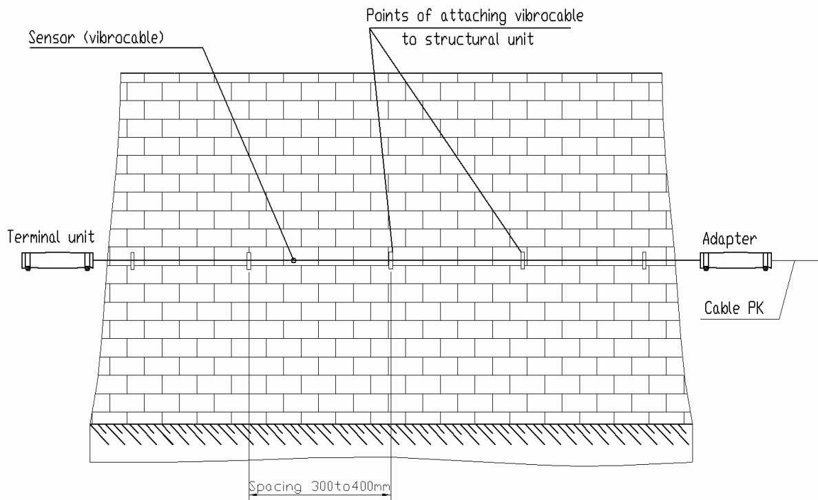
Variant 1. Sensor laid unconcealed and fastened with brackets
